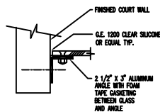
DETAIL 1 (ALTERNATE SIDE WALL CONFIGURATION)
