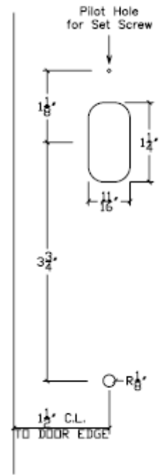
High Security Hasp Door Routes
