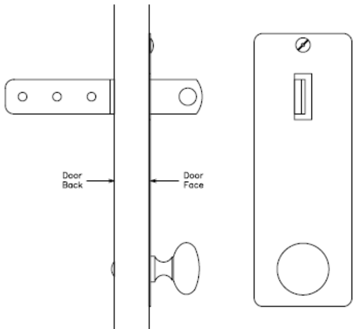
High Security Hasp Set Up
